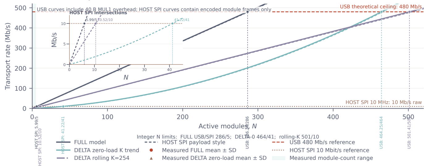
(c) Total transport rate and link limits at 200 Hz
